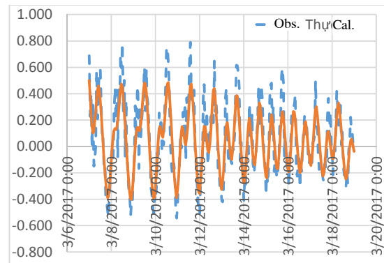
Fig. 8. Calculated and measured water levels at TamAnh station in 2017.
