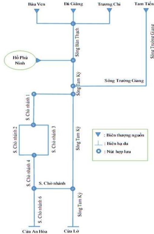
Fig. 3. 1D hydraulic diagram MIKE11 for Tam Ky river.
