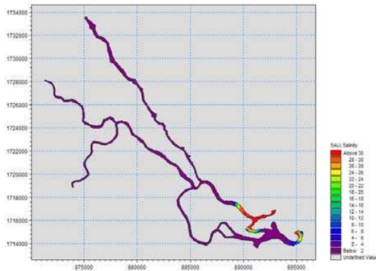
Fig. 10. Result of salinity spread across the whole region at 2pm on 9/11/2001.
