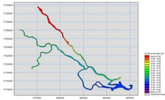
Fig. 9. Result at the water level in the whole region at 5pm on 11/11/2001.
