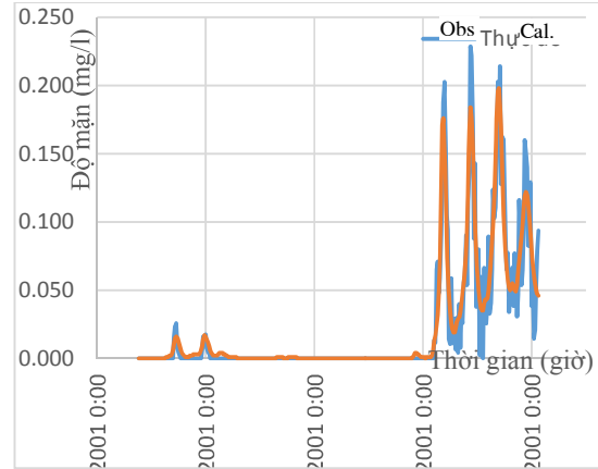
Fig. 7. Salinization at Tam Anh station from 11/8/2001 to 23/8/2001.
